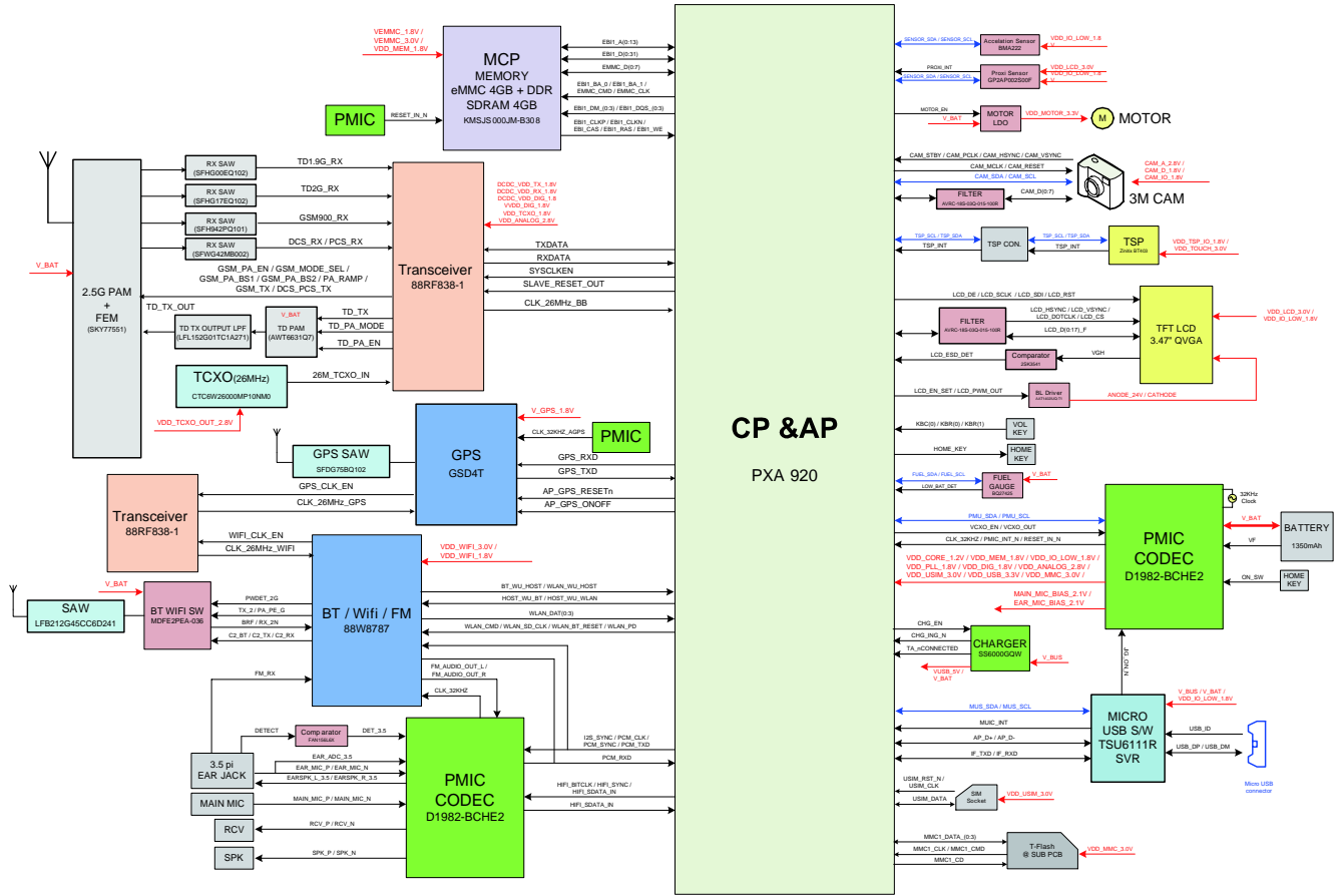
GT-S6358 Rev0.3 BLOCK DIAGRAM
