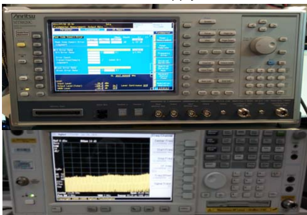
↑ MT8820C & Spectrum Analyzer
